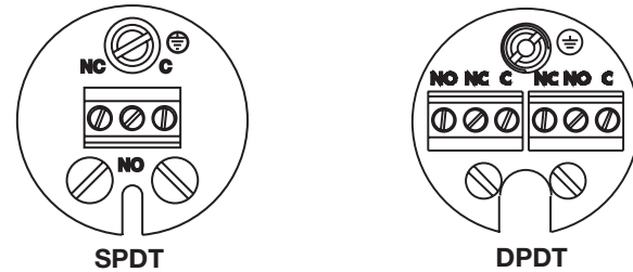
TERMINAL CONNECTIONS
